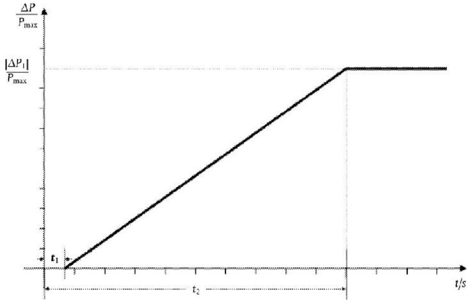
Figure 2: Active power frequency response capability of an HVDC system. \frac{|\Delta P_1|}{P_{\max}} is the change in active power triggered by the step change in frequency.
